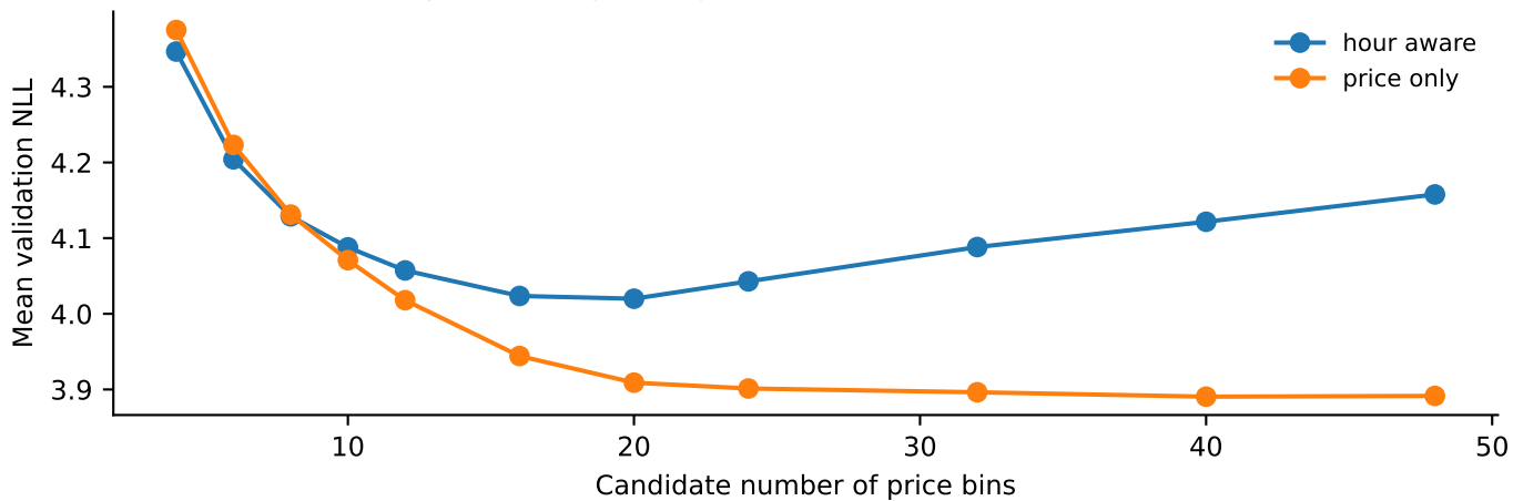
B. Synthetic expanding-window model selection (30 seeds)
